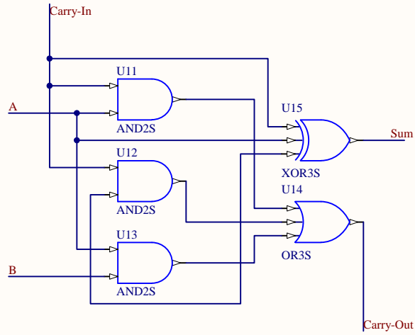
1-Bit Adder - Logic
