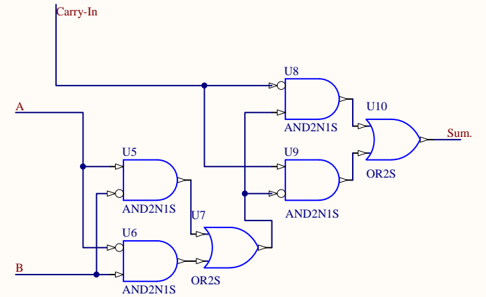
1-Bit Adder - Sum Logic
