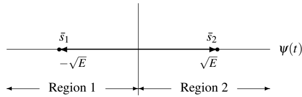
Figure 1: 2-signal point constellation for BPSK.
